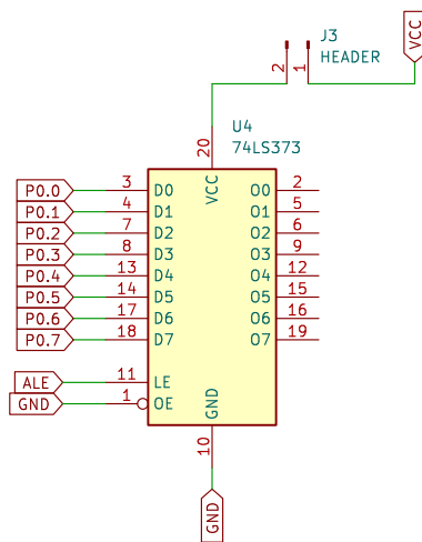
74LS373 Latch
